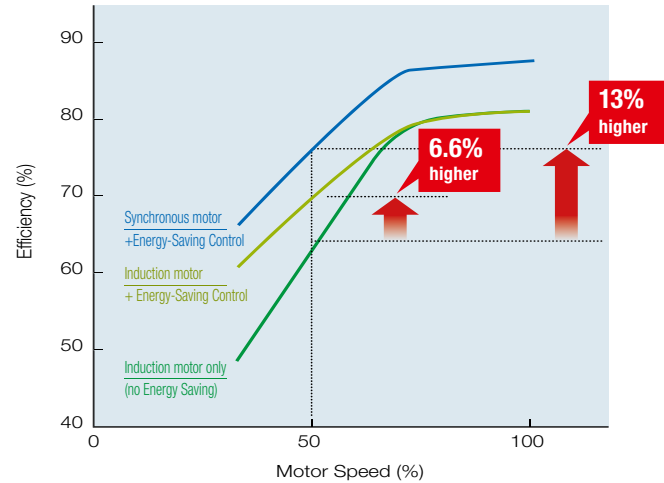
Efficiency with energy saving function Example shows a 200 V 4.0 kW drive in a fan or pump application
